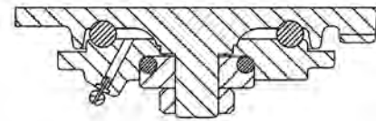
68 Series Cross Sectional View (Optional)
